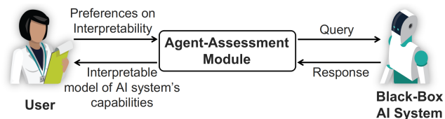
Figure 1: The agent-assessment module uses its user’s preferred vocabulary, queries the AI system, and delivers a user-interpretable causal model of the AI system’s capabilities. The AI system does not need to know the user’s vocabulary or modeling language.
