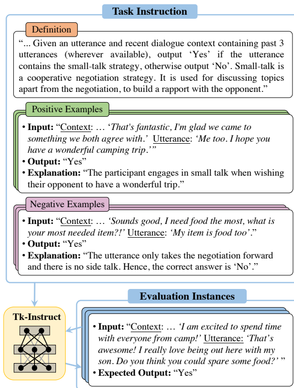
Figure 1: An example task from SUP-NATINST adopted from Chawla et al. (2021). A successful model is expected to use the provided instructions (including task definition and demonstration examples) to output responses to a pool of evaluation instances.
